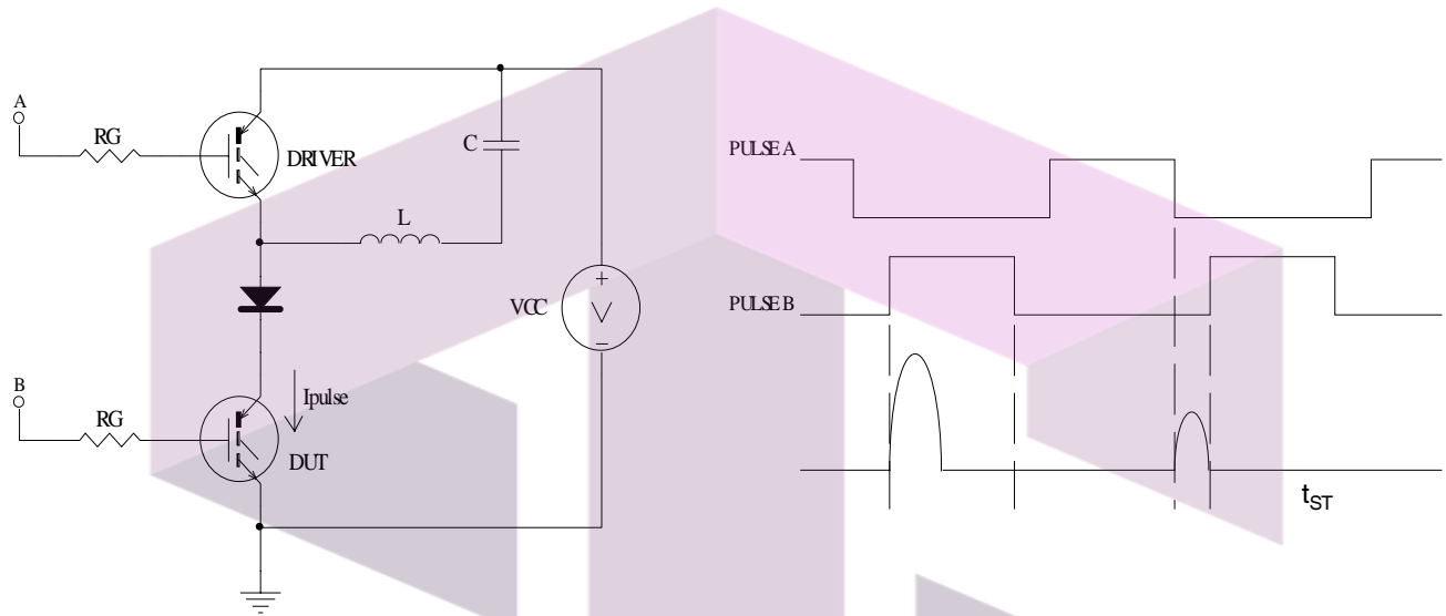
Fig 16a. t_{st} and E_{PULSE} Test Circuit
